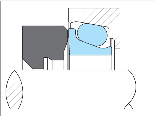
Figure 3 Special Design
