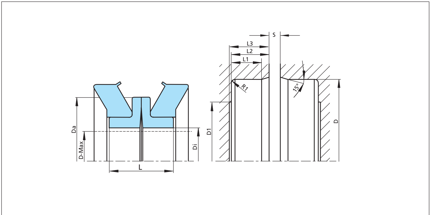
Figure 11 Installation Drawing
